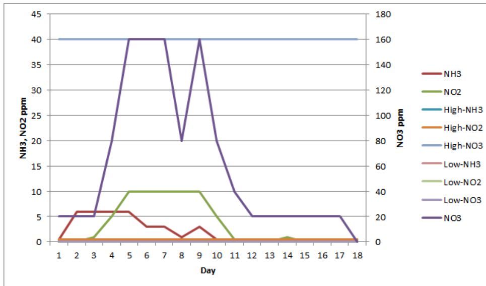
Figure 1. This graph represents the amounts/levels of NH3, NO2, and NO3.
