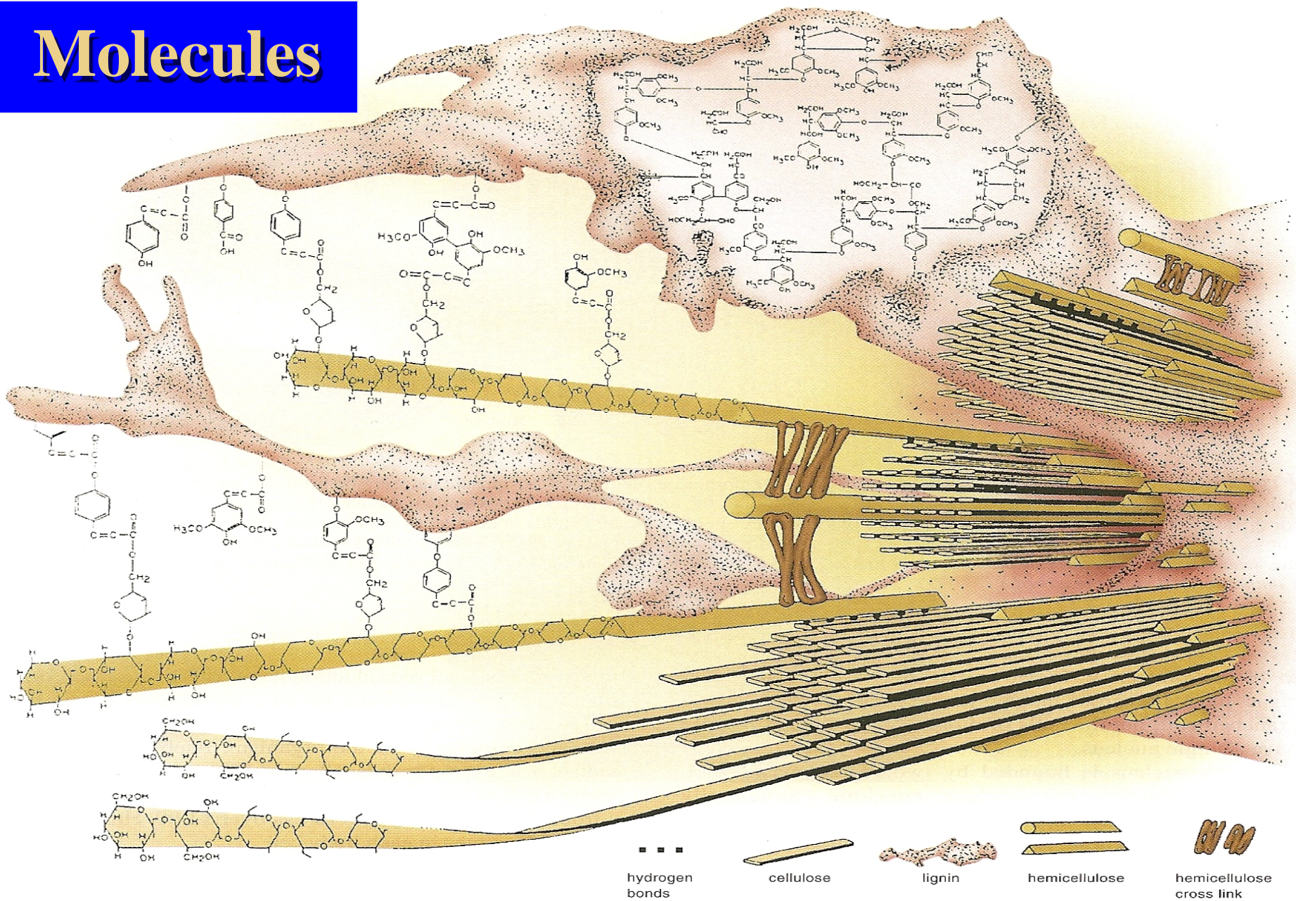
Figure 3.6B Secondary cell wall structure. Components are arranged so that the cellulose microfibrils and hemicellulose chains are embedded in lignin. (Reproduced by permission of the Oklahoma Academy of Science; Figure provided by Dr. James E. Bidlack.)
